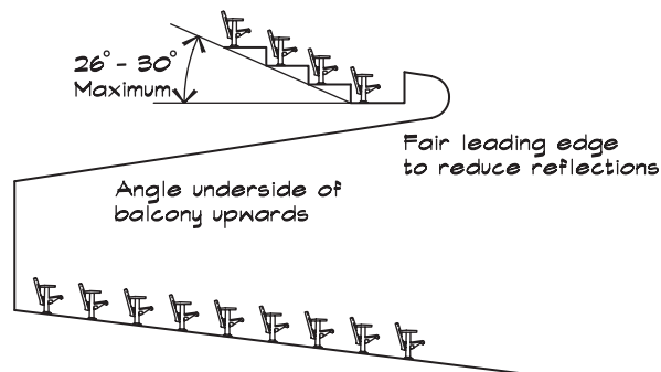
FIGURE 20.2 Balcony Design
