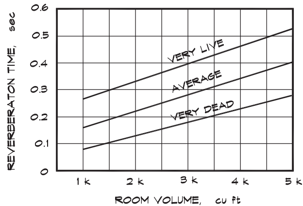
FIGURE 21.9 Suggested Reverberation Times for Control Rooms (Fierstein, 1979)
