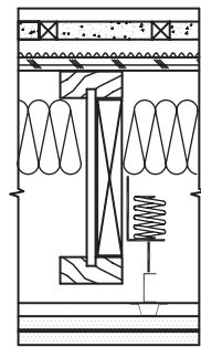
FIGURE 15.14 Double Isolated Wood Floor–Ceiling (Adams, 2002)
