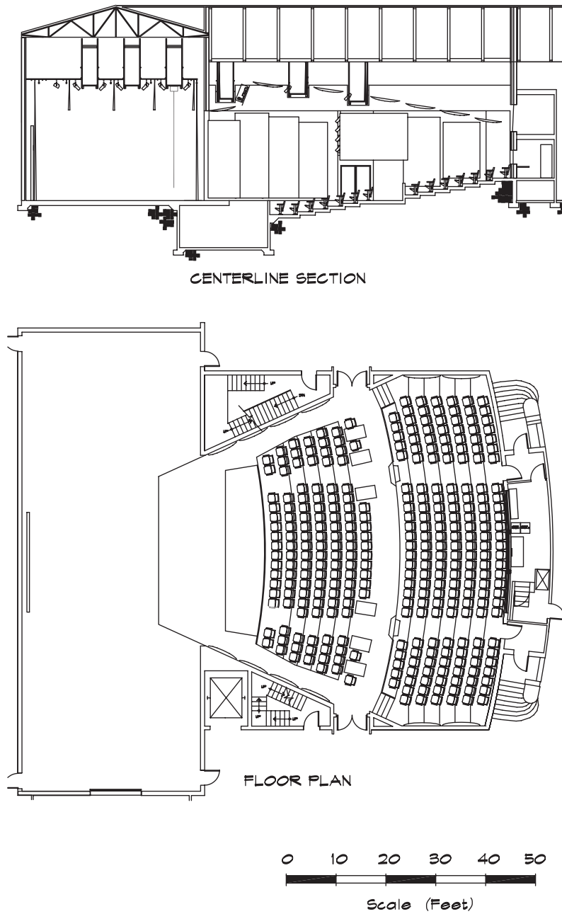
FIGURE 20.7 Meadows School Auditorium, Las Vegas, NV, USA (Acoustician: Marshall Long Acoustics) (Architect: Killefer, Flammang, Purtil)
