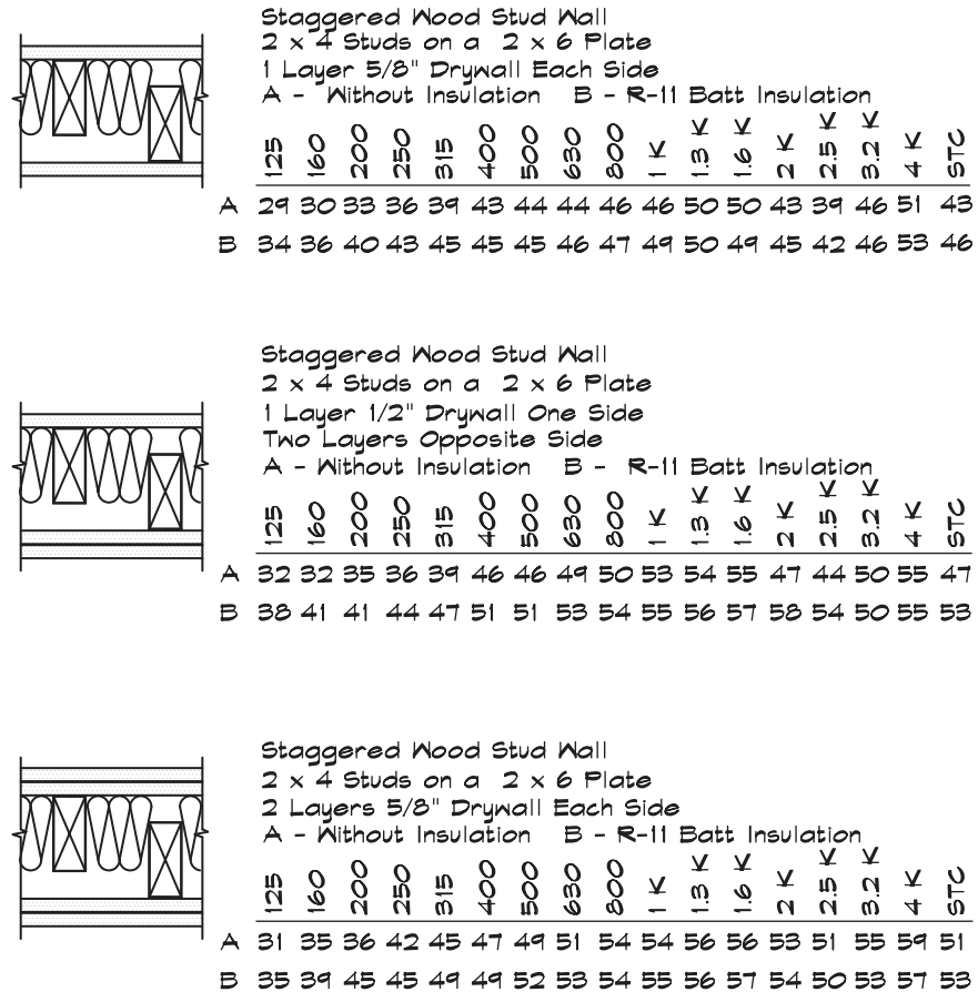
FIGURE 10.8 Transmission Loss of Staggered Stud Walls (California Office of Noise Control, 1981)
