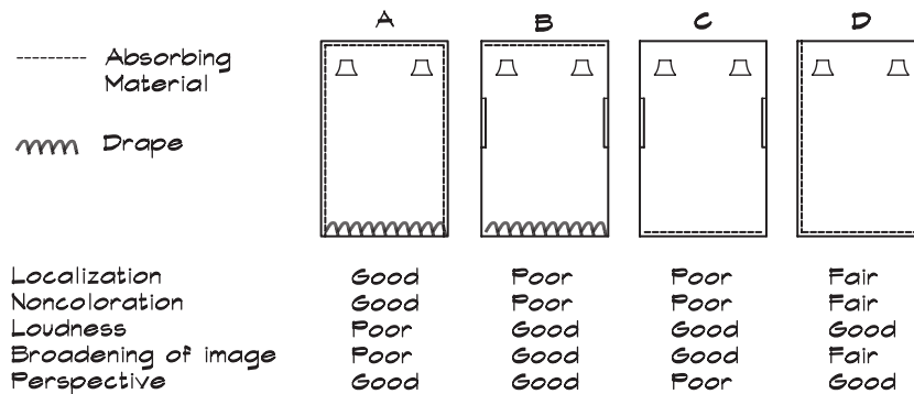
FIGURE 21.14 Summary of the Results of the Nippon Gakki Listening Tests (Kishinaga et al., 1979)
