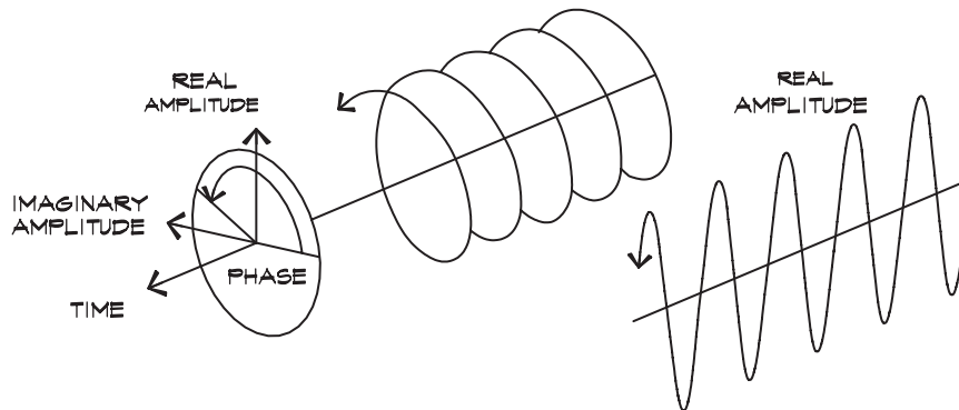
FIGURE 2.7 Sine Wave in Time and Phase Space
