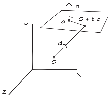
FIGURE 22.9 Ray-Plane Intersection
