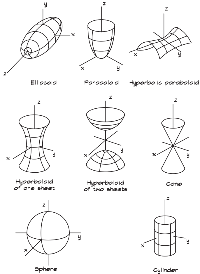
FIGURE 22.12 Quadric Surfaces
