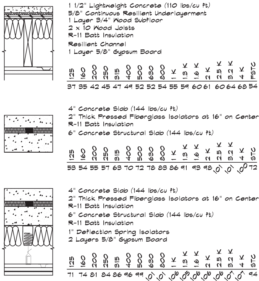
FIGURE 12.5 Transmission Loss of Floating Floors (Kinetics Corporation Test Data)
