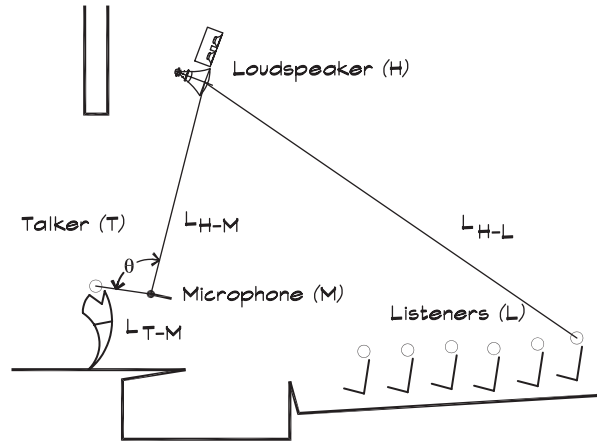
FIGURE 18.11 Parameters for Feedback Control
