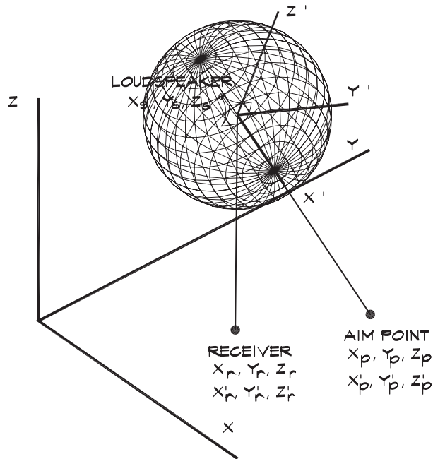
FIGURE 18.26 Loudspeaker Coordinate System
