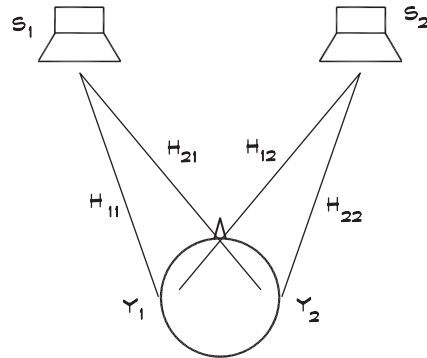
FIGURE 22.28 Binaural Reproduction Using Stereo Loudspeakers (Schroeder and Atal, 1963)
