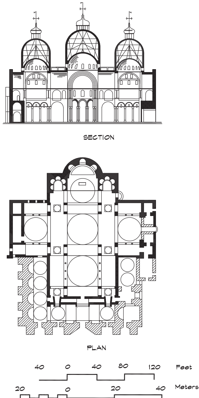
FIGURE 1.7 St. Mark's Cathedral, Venice, Italy (Fletcher, 1963)
