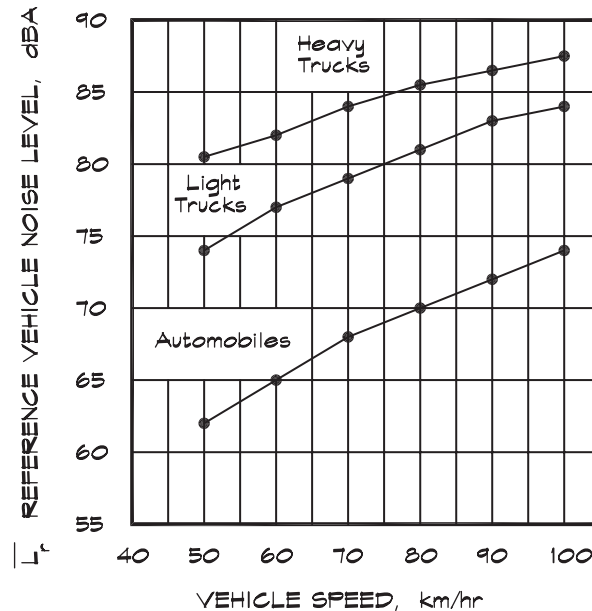
FIGURE 5.26 Reference Energy Mean Vehicle Emission Levels (Barry and Reagan, 1978)
