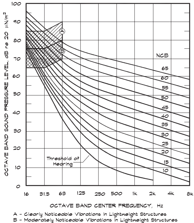
FIGURE 4.21 Balanced Noise Criterion Curves (NCB) (Beranek, 1989)
