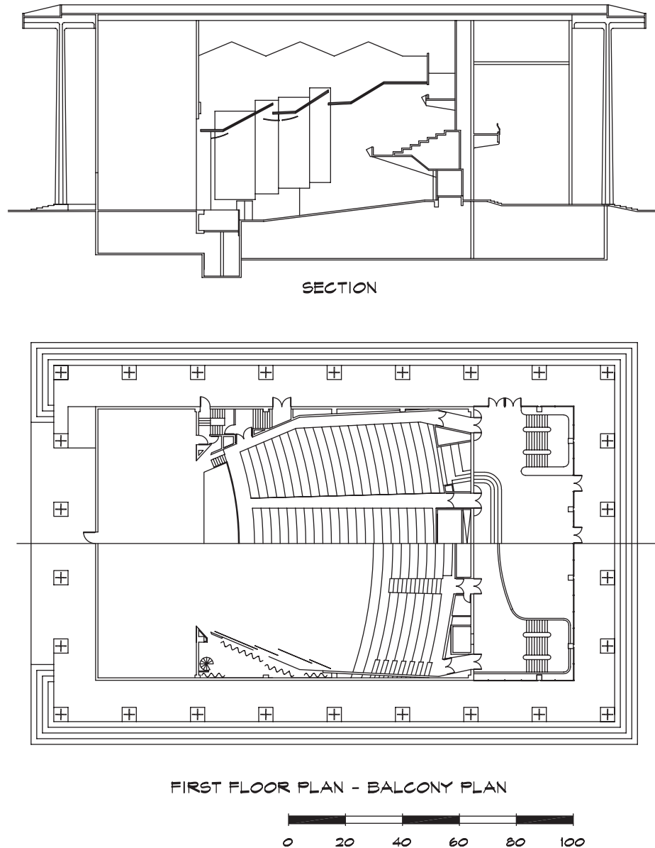
FIGURE 20.9 Ambassador College Auditorium, Pasadena, CA, USA (Acoustician: BBN; Architect: DMJM)
