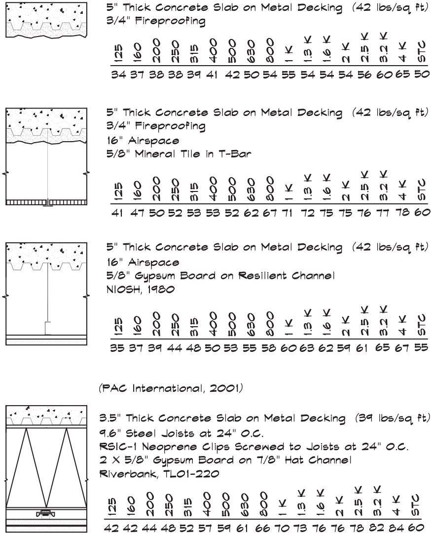
FIGURE 12.1 Transmission Loss of Metal Deck Floor-Ceilings (National Research Council Canada, 1966)
